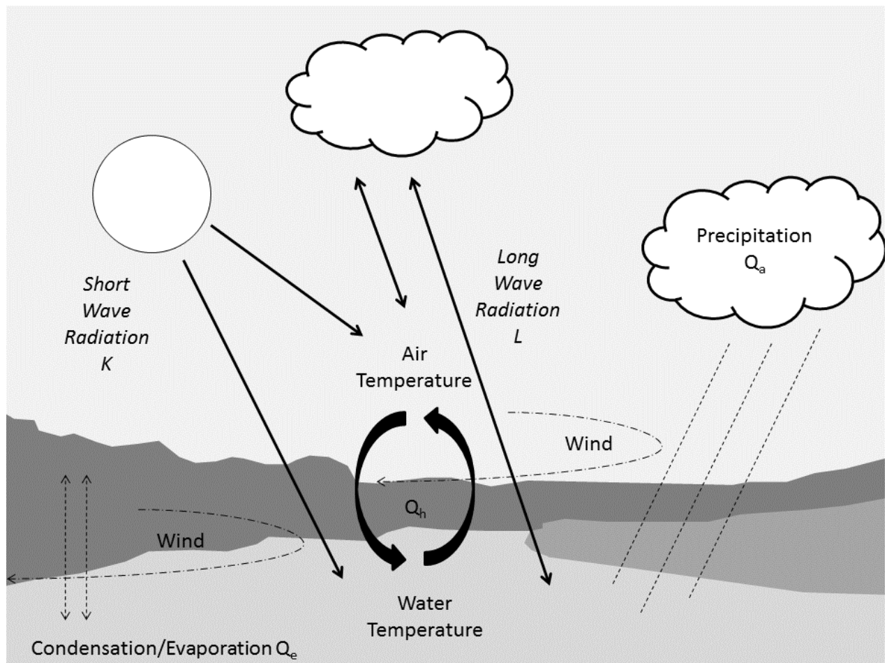
Figure 1. Multiple interdependent climate controls of water temperature; Q^* is the sum of K and L ; Q_a also small advective fluxes due to inflow/outflow into river, hyporheic exchange, groundwater (not shown); [adapted from Caissie (2006) and Hannah et al. (2008)].
