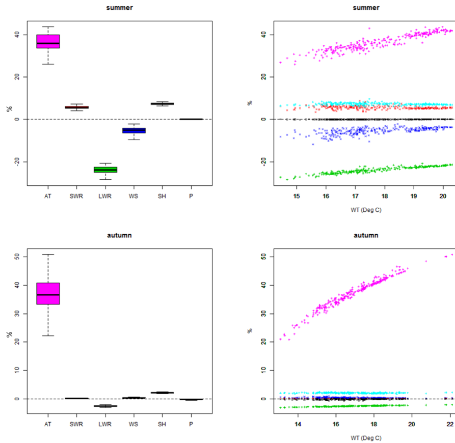
1 2 Figure 5b. Contributions of climate predictors to modelled WT (summer and autumn): left- 3 hand side, boxplots of percentage contributions of climate predictors to modelled WT values 4 for all data-points (except outliers); right-hand side, scatter plots of percentage contributions 5 of climate predictors to modelled WT values against modelled WT values for all data-points; 6 colour-coding for all plots: magenta, AT; red, SWR; green, LWR; dark blue, WS; cyan, SH; 7 black, P.
