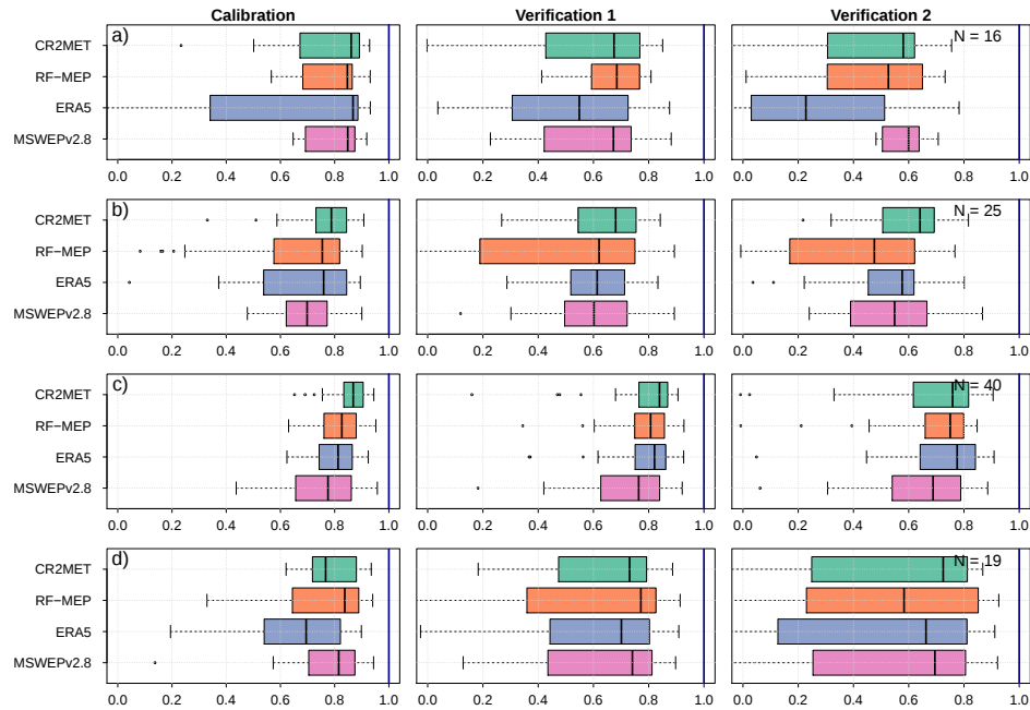
Figure 21. Performance of TUWmodel during calibration (2000–2014), Verification 1 (1990–1999) and Verification 2 (2015–2018), prior to any regionalisation over catchments with different hydrological regimes: a ) snow-dominated; b ) Nivo-pluvial; c ) pluvio-nival; and d ) rain-dominated.
