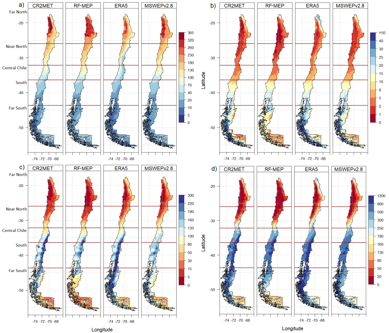
Figure R5. Median annual values of four Climdex indices over 1990–2018 (full period): a ) number of consecutive dry days (CDD); b ) number of consecutive wet days (CWD); c ) maximum P over five consecutive days (RX5day); and d ) annual P accumulated for events that are above the 95th percentile of the daily P for wet days (R95pTOT). The dark red horizontal lines represent the limits of each macroclimatic zone.
