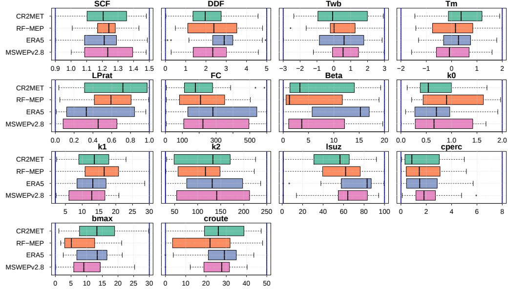
Figure R13. Model parameters obtained through calibration in rain-dominated catchments. The vertical blue lines indicate the upper and lower limits of the parameter ranges.
