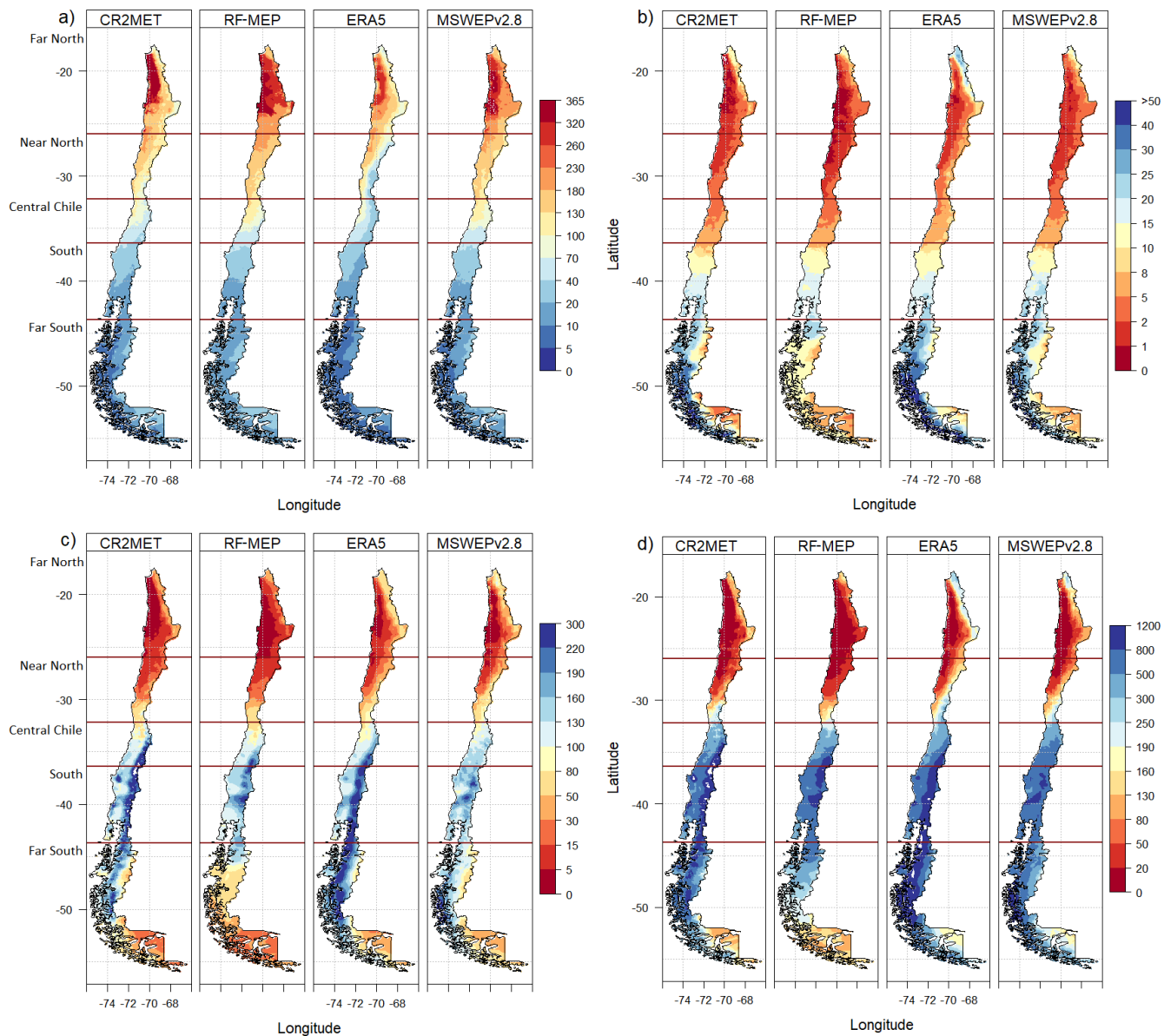
Figure R6. Median annual values of four Climdex indices over 2000–2014 (near-normal): a ) number of consecutive dry days (CDD); b ) number of consecutive wet days (CWD); c ) maximum P over five consecutive days (RX5day); and d ) annual P accumulated for events that are above the 95th percentile of the daily P for wet days (R95pTOT). The dark red horizontal lines represent the limits of each macroclimatic zone.
