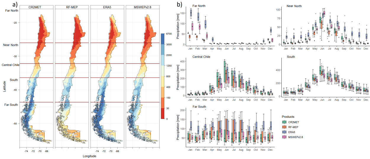
Figure R1. Comparison of P products over 1990–2018 (full time period): a ) mean annual P for each product resampled to a 0.05^\circ spatial resolution using the nearest neighbour method. The dark red horizontal lines represent the limits of each major macroclimatic zone; and b ) mean monthly P averaged over each catchment located within each macroclimatic zone (see Figure 1d).
