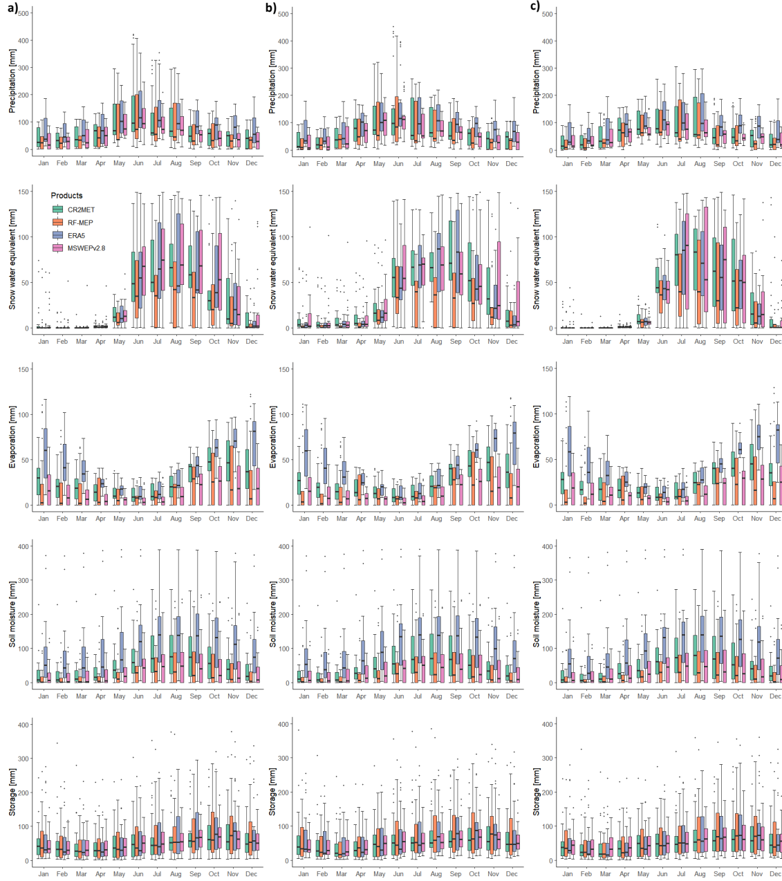
Figure R15. Mean monthly water balance components over nivo-pluvial catchments, obtained by forcing the TUW model with different P products for the: a ) calibration (2000–2014); b ) Verification 1 (1990–1999); and c ) Verification 2 (2015–2018) periods. Mean monthly P was added for comparison purposes.
