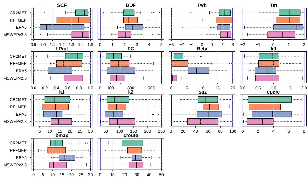
Figure R11. Model parameters obtained through calibration in nivo-pluvial catchments. The vertical blue lines indicate the upper and lower limits of the parameter ranges.
