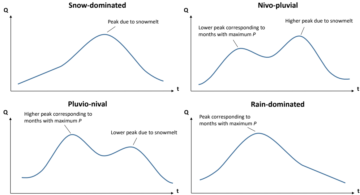
Figure 22. Conceptual illustration of the hydrological regimes used to classify the 100 near-natural catchments used in this study.
