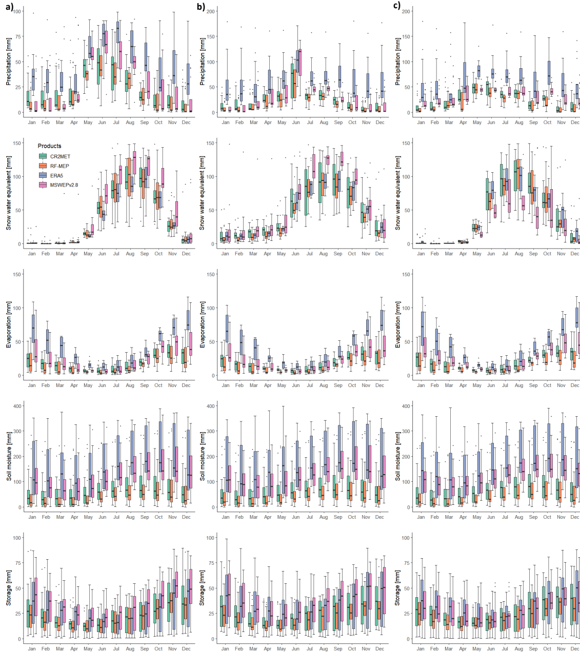
Figure R14. Mean monthly water balance components over snow-dominated catchments, obtained by forcing the TUV model with different P products for the: a ) calibration (2000–2014); b ) Verification 1 (1990–1999); and c ) Verification 2 (2015–2018) periods. The mean monthly P was added for comparison purposes.
