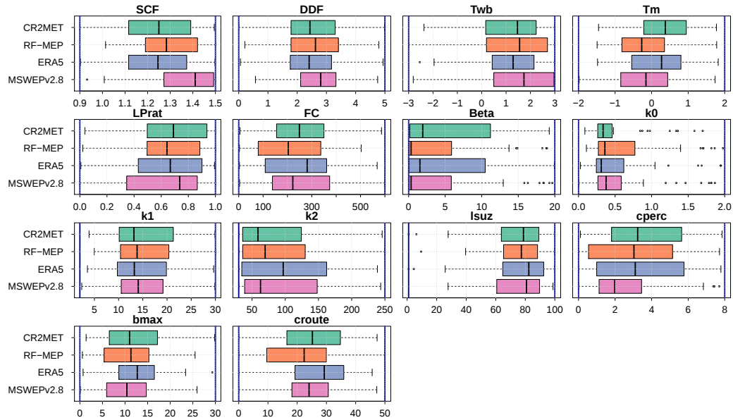
Figure R26. Model parameters obtained through calibration of catchments located in the South region. The vertical blue lines indicate the upper and lower limits of the parameter ranges.
