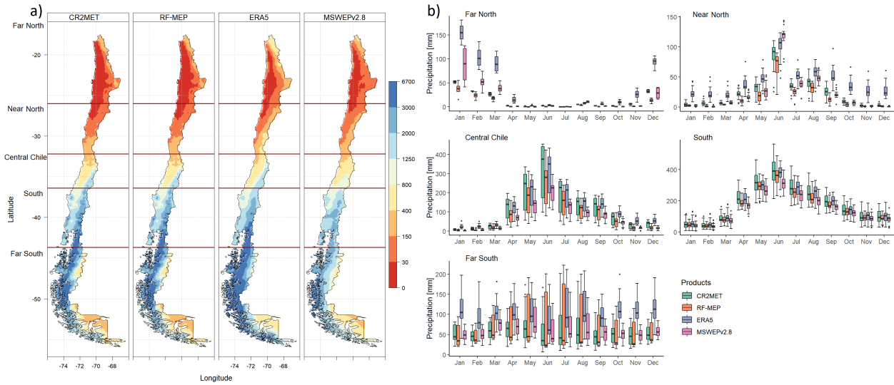
Figure R3. Comparison of P products over 1990–1999 (near-normal): a ) mean annual P for each product resampled to a 0.05^\circ spatial resolution using the nearest neighbour method. The dark red horizontal lines represent the limits of each major macroclimatic zone; and b ) mean monthly P averaged over each catchment located within each macroclimatic zone (see Figure 1d).
