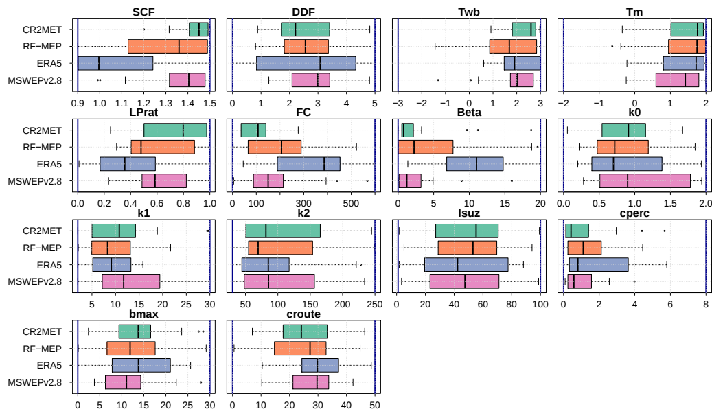
Figure R27. Model parameters obtained through calibration of catchments located in the Far South region. The vertical blue lines indicate the upper and lower limits of the parameter ranges.
