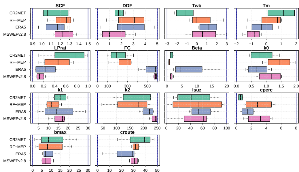
Figure R23. Model parameters obtained through calibration of catchments located in the Far North region. The vertical blue lines indicate the upper and lower limits of the parameter ranges.
