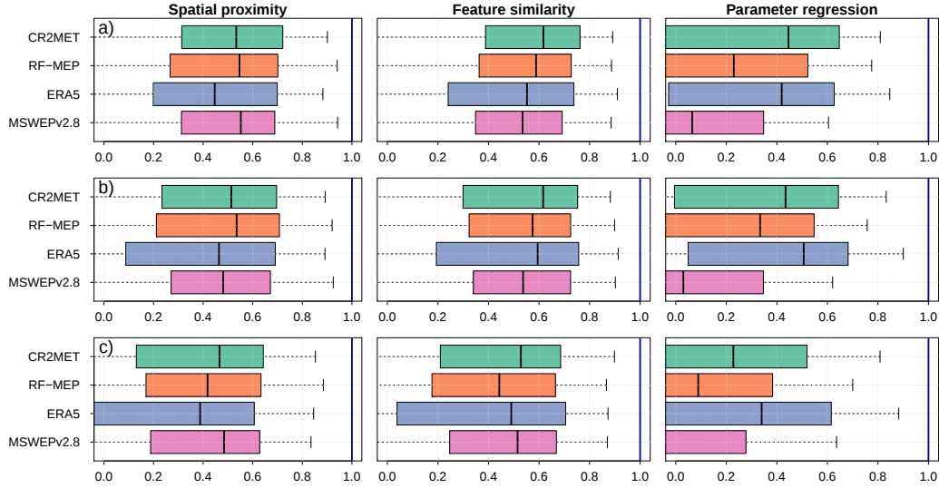
Figure R9. Leave-one-out cross-validation results for the three regionalisation methods applied with different P products during the: a) calibration (2000–2014); b) Verification 1 (1990–1999); and c) Verification 2 (2015–2018) periods.
