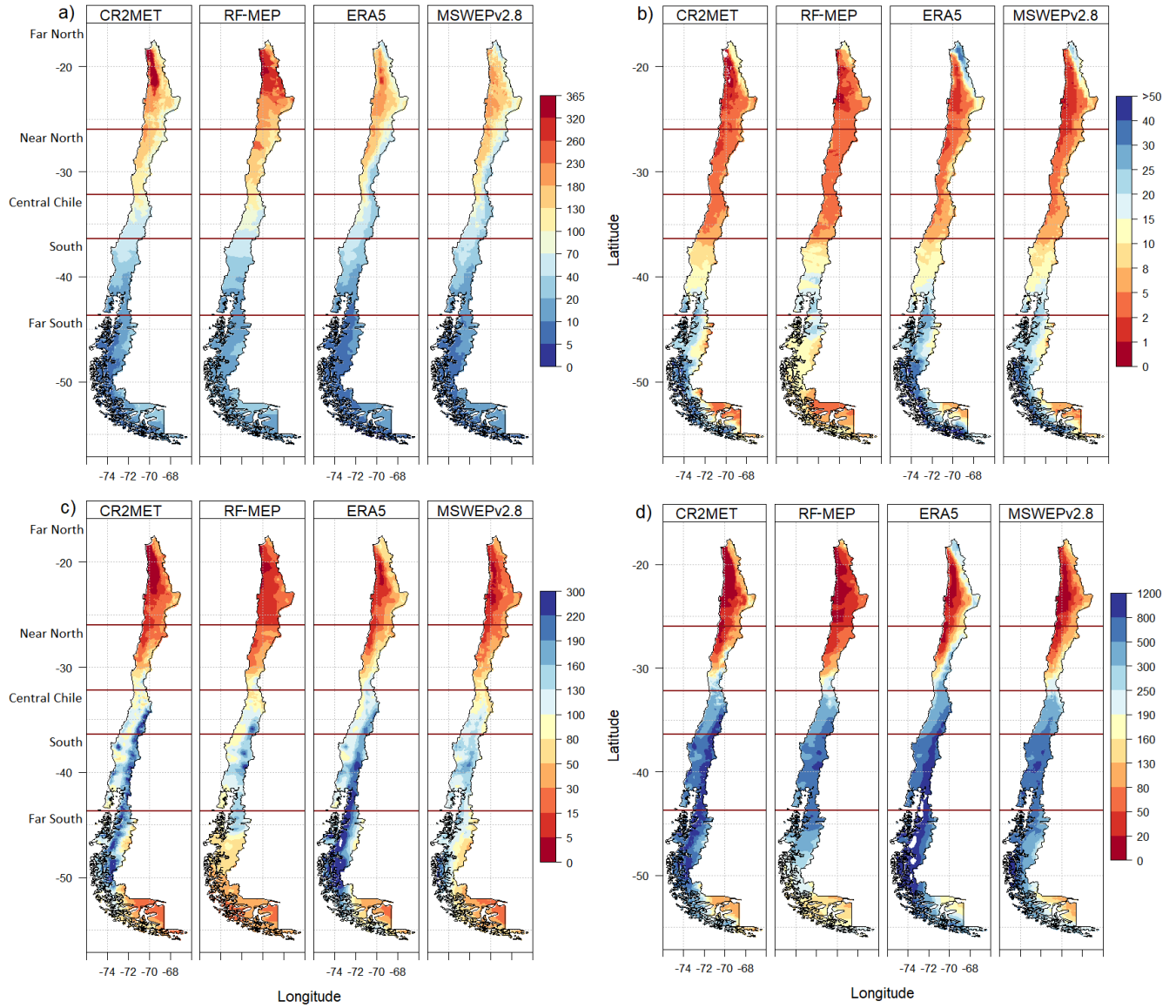
Figure R8. Median annual values of four Climdex indices over 2015–2018 (dry): a ) number of consecutive dry days (CDD); b ) number of consecutive wet days (CWD); c ) maximum P over five consecutive days (RX5day); and d ) annual P accumulated for events that are above the 95th percentile of the daily P for wet days (R95pTOT). The dark red horizontal lines represent the limits of each macroclimatic zone.
