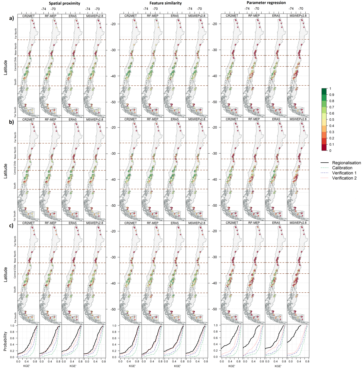
Figure R19. Spatial performance of the leave-one-out cross-validation results for the three regionalisation methods according to P product used to force TUWmodel. Results are presented for the: a ) calibration (2000–2014); b ) Verification 1 (1990–1999); and c ) Verification 2 (2015–2018) periods. The panels beneath the map plots refer to the ECDFs of the corresponding regionalisation technique for the entire period of analysis (1990–2018) and P product (black) against the performances during the independent calibration (green), Verification 1 (blue), and Verification 2 (red) periods.
