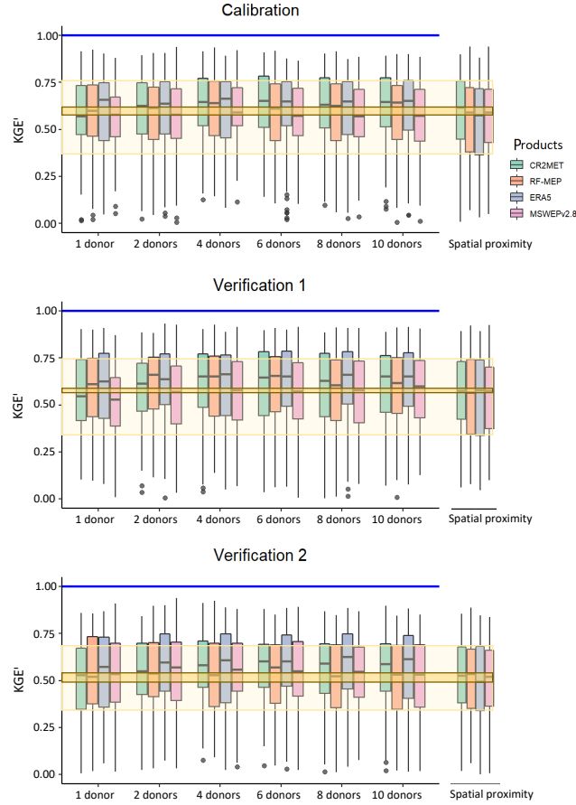
Figure R18. Influence of the number of donors used for feature similarity for calibration (2000—2014); Verification 1 (1990–1999); and Verification 2 (2015–2018). The results from spatial proximity are included on the right of each panel for comparison purposes. The dark yellow box denotes the upper and lower bounds of the median performance (of the four P products) obtained with spatial proximity, while the lighter yellow box represents the upper and lower bounds of the interquartile range for spatial proximity.
