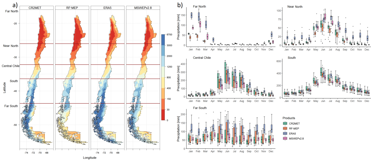
Figure R2. Comparison of P products over 2000–2014 (near-normal): a ) mean annual P for each product resampled to a 0.05^\circ spatial resolution using the nearest neighbour method. The dark red horizontal lines represent the limits of each major macroclimatic zone; and b ) mean monthly P averaged over each catchment located within each macroclimatic zone (see Figure 1d).
