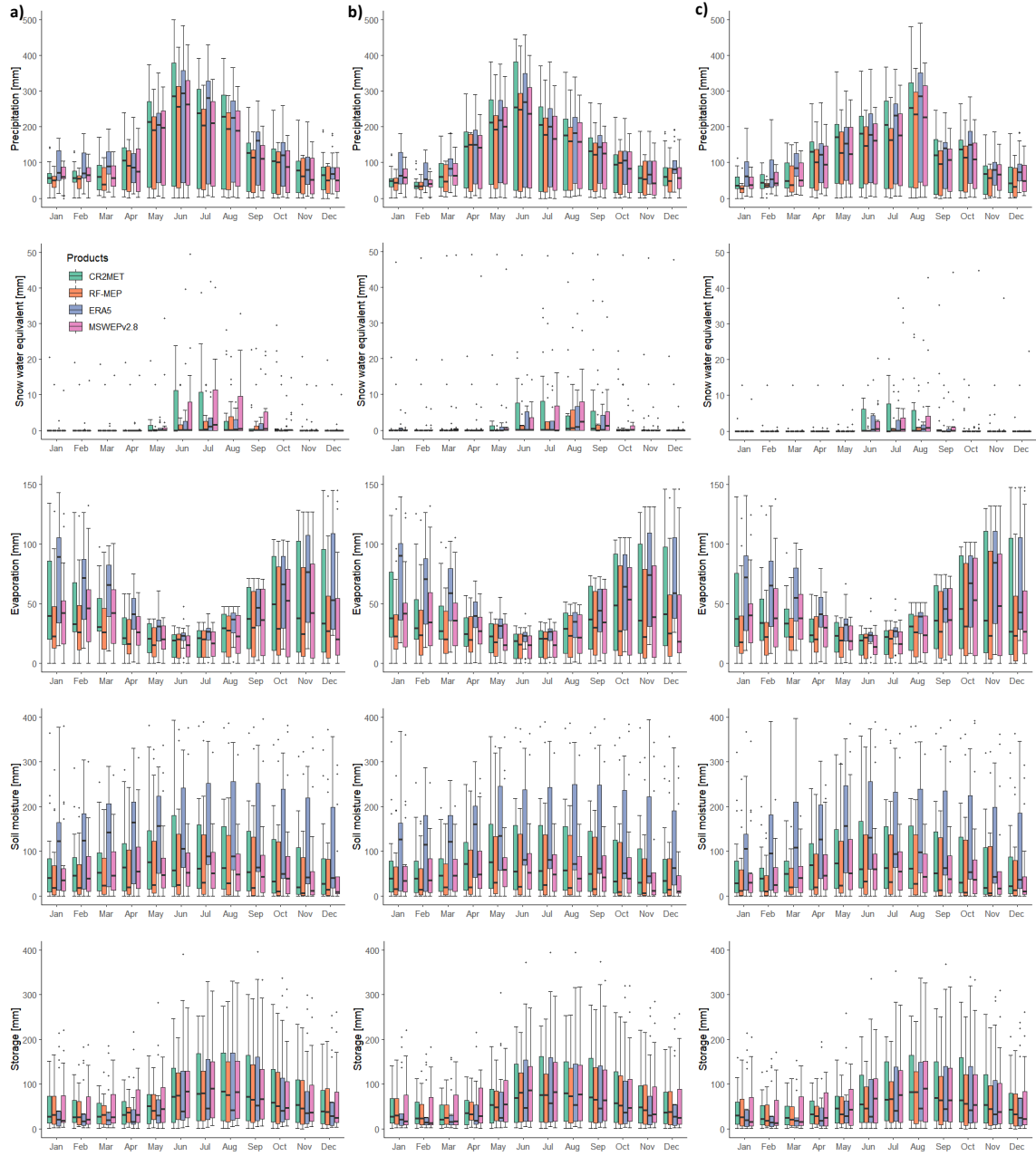
Figure R17. Mean monthly water balance components over rain-dominated catchments, obtained by forcing the TUW model with different P products for the: a ) calibration (2000–2014); b ) Verification 1 (1990–1999); and c ) Verification 2 (2015–2018) periods. The mean monthly P was added for comparison purposes.
