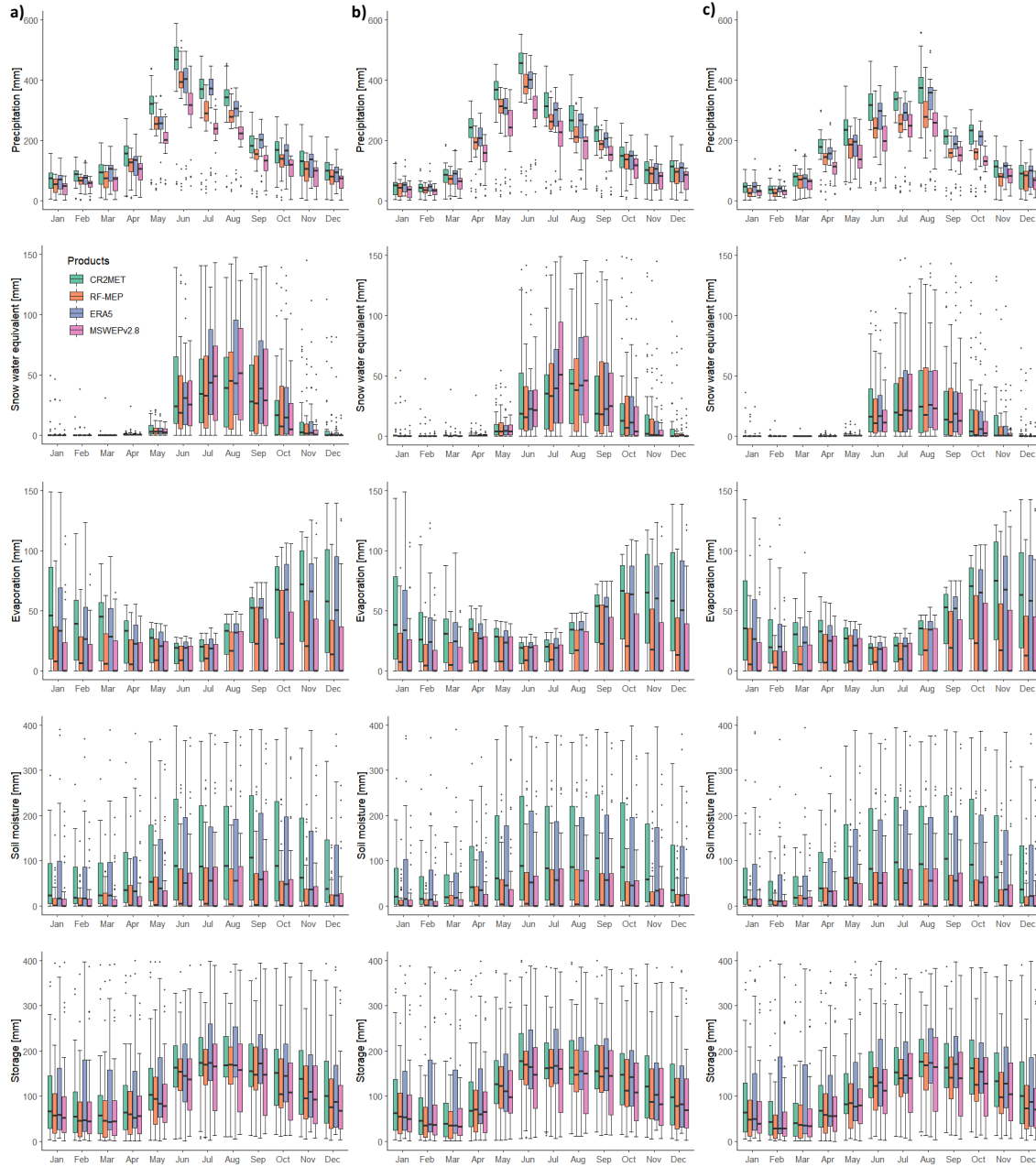
Figure R16. Mean monthly water balance components over pluvio-nival catchments, obtained by forcing the TUW model with different P products for the: a ) calibration (2000–2014); b ) Verification 1 (1990–1999); and c ) Verification 2 (2015–2018) periods. The mean monthly P was added for comparison purposes.
