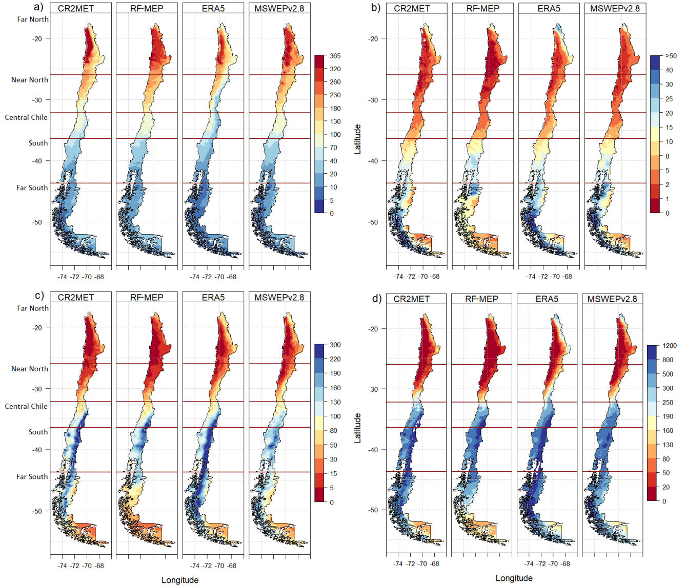
Figure R7. Median annual values of four Climdex indices over 1990–1999 (near-normal): a ) number of consecutive dry days (CDD); b ) number of consecutive wet days (CWD); c ) maximum P over five consecutive days (RX5day); and d ) annual P accumulated for events that are above the 95th percentile of the daily P for wet days (R95pTOT). The dark red horizontal lines represent the limits of each macroclimatic zone.
