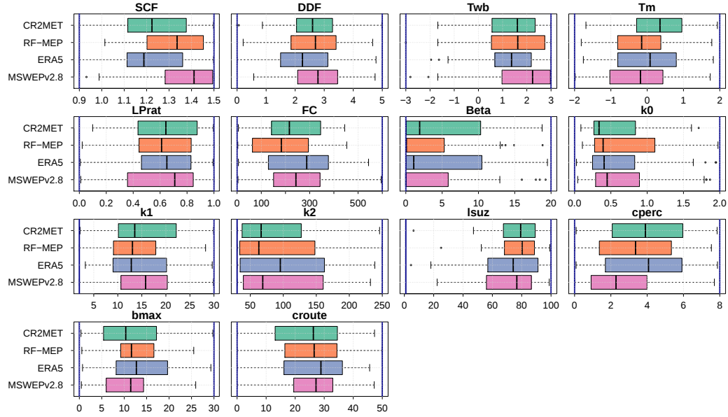
Figure R12. Model parameters obtained through calibration in pluvio-nival catchments. The vertical blue lines indicate the upper and lower limits of the parameter ranges.
