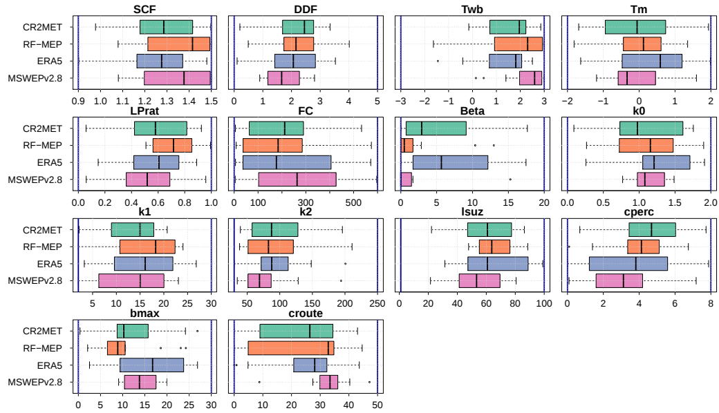
Figure R25. Model parameters obtained through calibration of catchments located in Central Chile. The vertical blue lines indicate the upper and lower limits of the parameter ranges.
