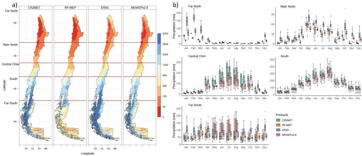
Figure R4. Comparison of P products over 2015–2018 (dry): a ) mean annual P for each product resampled to a 0.05^\circ spatial resolution using the nearest neighbour method. The dark red horizontal lines represent the limits of each major macroclimatic zone; and b ) mean monthly P averaged over each catchment located within each macroclimatic zone (see Figure 1d).
