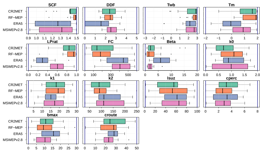
Figure R10. Model parameters obtained through calibration in snow-dominated catchments. The vertical blue lines indicate the upper and lower limits of the parameter ranges.
