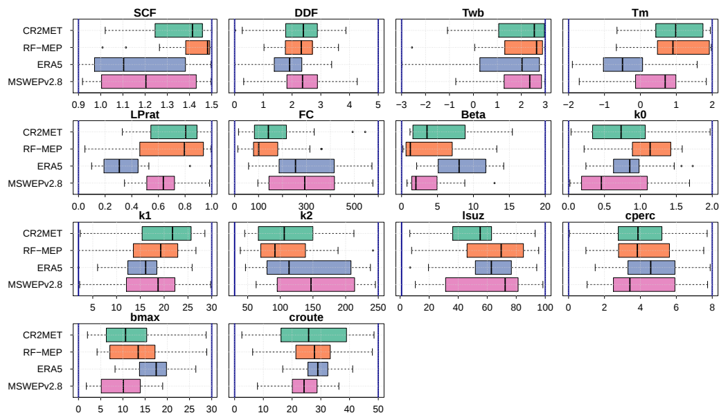
Figure R24. Model parameters obtained through calibration of catchments located in the Near North region. The vertical blue lines indicate the upper and lower limits of the parameter ranges.
